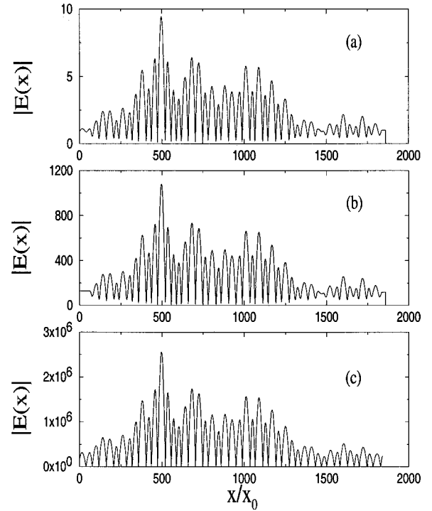
FIG. 2. Amplitude of the electric field of the 30-cell system vs x/x_0 , with x_0 = 5 nm, for the peak P_2 in Fig. 1a. (a) Without gain, incident field E_{inc} = 1 V/m; (b) with near-threshold gain ( P_r = 7.2 \times 10^6/s ), incident field E_{inc} = 1 V/m; (c) the lasing field with over-threshold pumping rate ( P_r = 2 \times 10^7/s ). Both (a) and (b) are obtained by the transfer matrix method while (c) is obtained by the FDTD method and laser theory.
