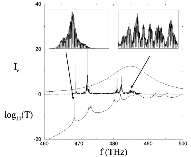
FIG. 3. Logarithm of the transmission coefficient T , the emission intensity I_e , and the gain profile vs frequency f for a 80-cell random systems. In the inset, wave functions of two modes are shown.
