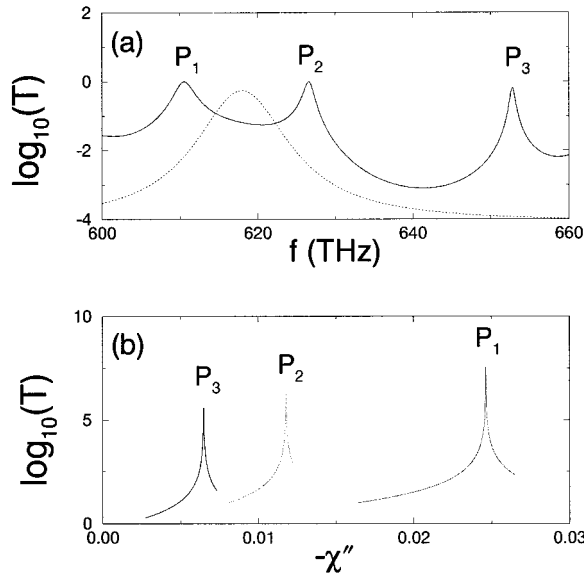
FIG. 1. (a) Logarithm of transmission coefficient vs frequency of a 30-cell random system with three typical peaks. The dotted line shows the frequency dependence of the gain profile. (b) Logarithm of the transmission coefficient vs \chi'' for the three peaks shown in (a) with a frequency-independent gain. \chi'' is proportional to the pumping rate P_r .
